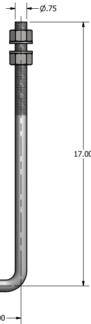
Ø.75 X 20.00 ANCHOR BOLT
